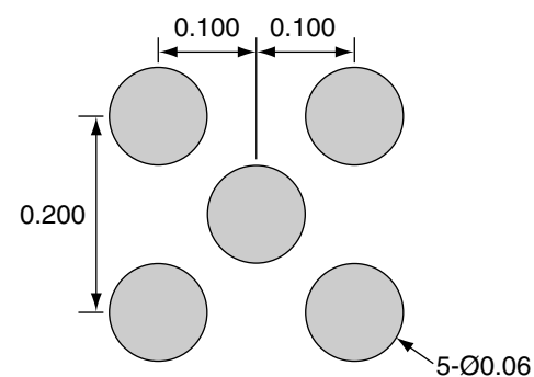
RECOMMENDED FOOTPRINT
